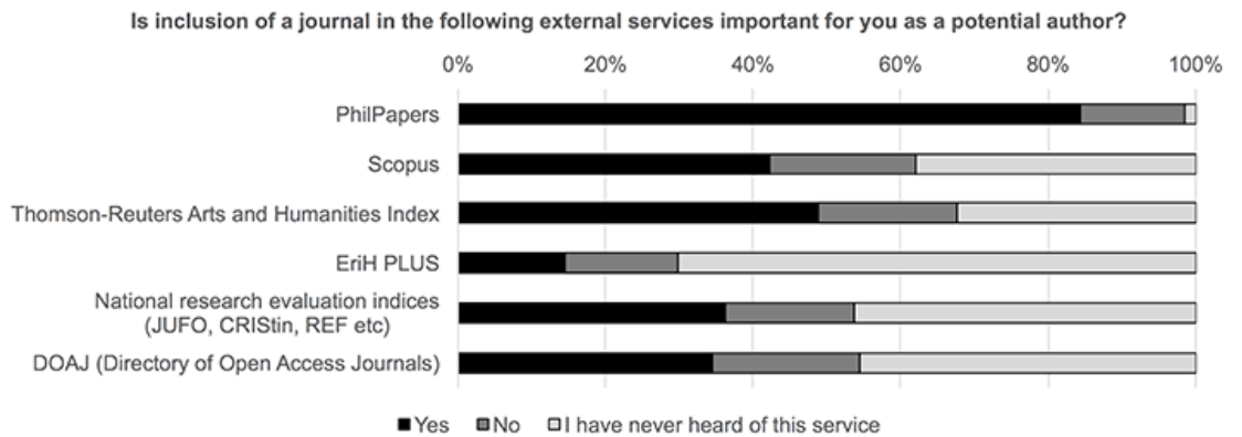
Figure 7: Indexing needs
